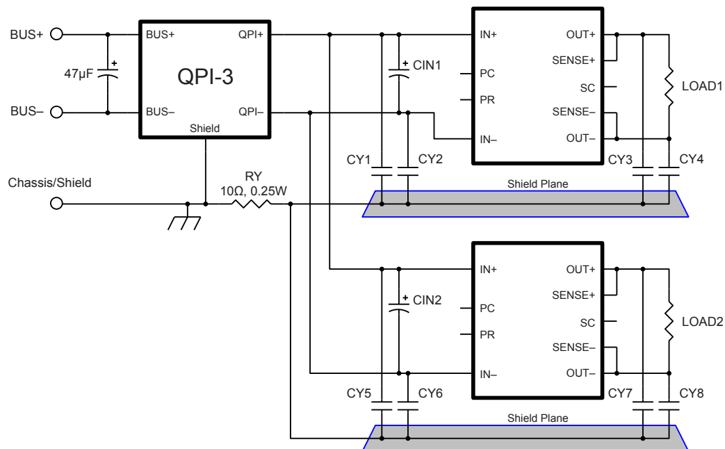
Figure 9 — The QPI-3 filtering dual supplies, using a single RY resistor [d]
