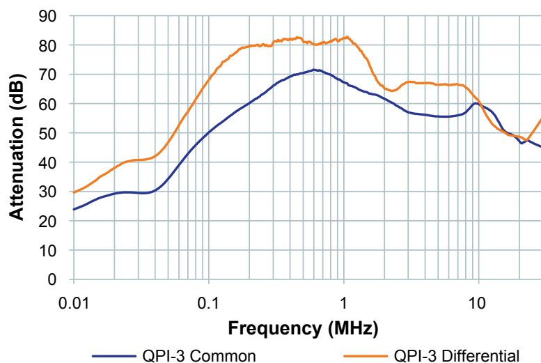
Figure 13 — Attenuation curves into a 50Ω line impedance, bias from a 28V bus
