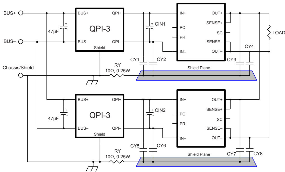
Figure 10 — Dual QPI-3's filtering paralleled converters feeding a common load [d]
