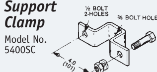
U-Bolt Assembly
