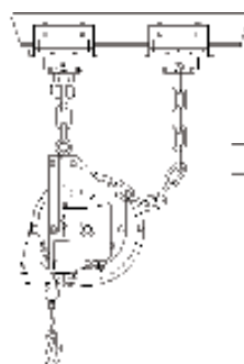
Trolley Mount
