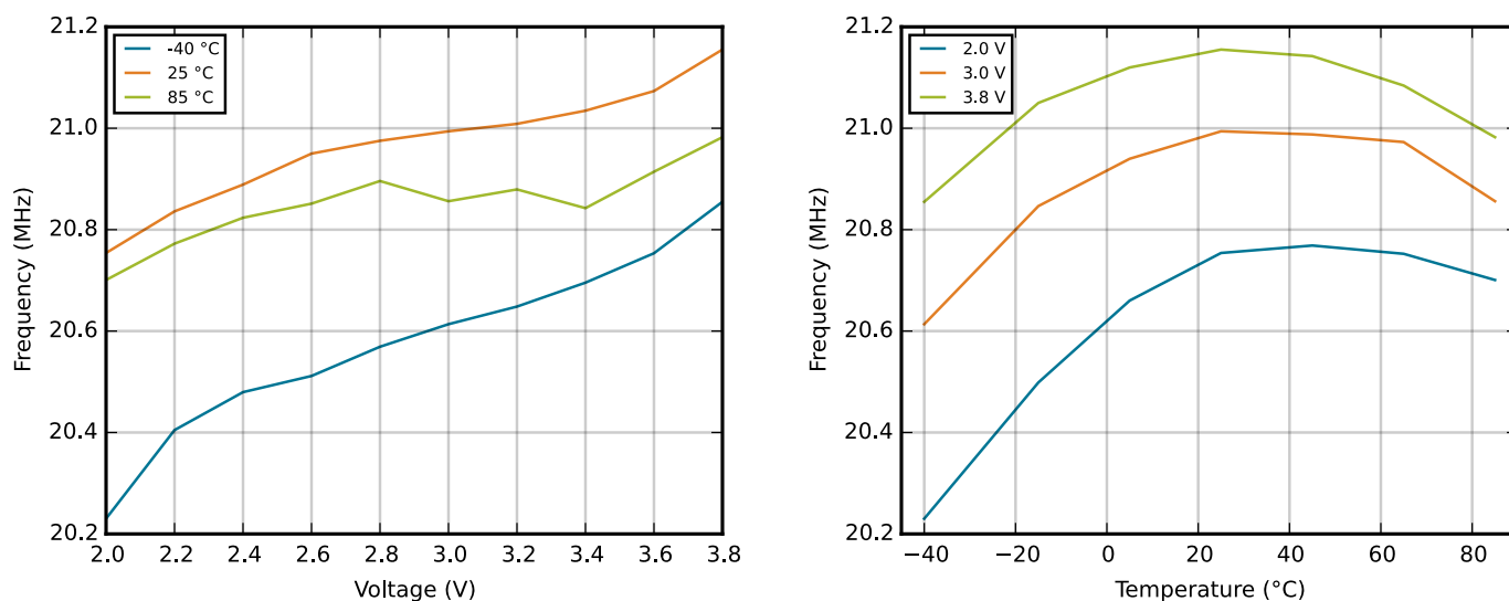
Figure 4.22. Calibrated HFCO 21 MHz Band Frequency vs Supply Voltage and Temperature
