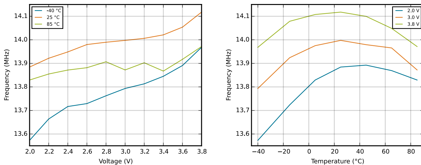
Figure 4.21. Calibrated HFCO 14 MHz Band Frequency vs Supply Voltage and Temperature
