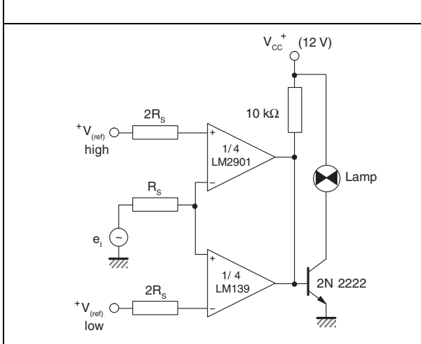
Figure 16. Limit comparator
