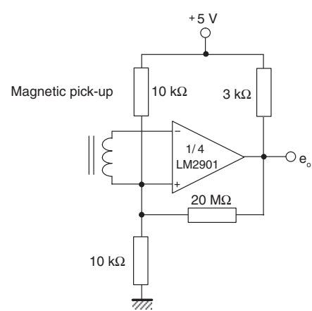
Figure 13. Transducer amplifier
