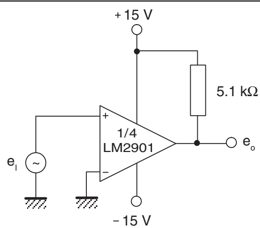
Figure 17. Split-supply applications - zero crossing detector
