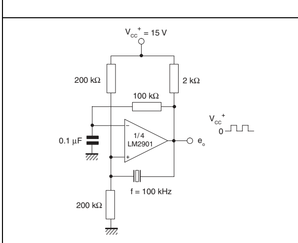
Figure 18. Crystal controlled oscillator
