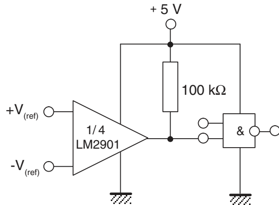
Figure 9. Driving CMOS
