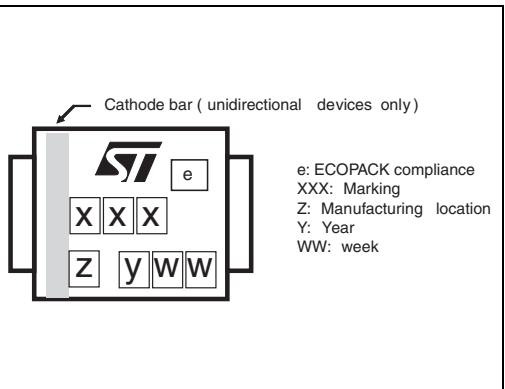
Figure 14. Marking layout (1)
