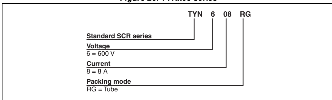
Figure 23. TYNx08 series
