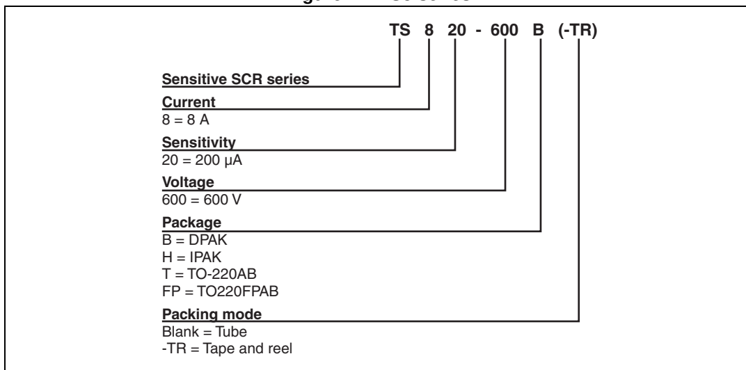
Figure 22. TS8 series
