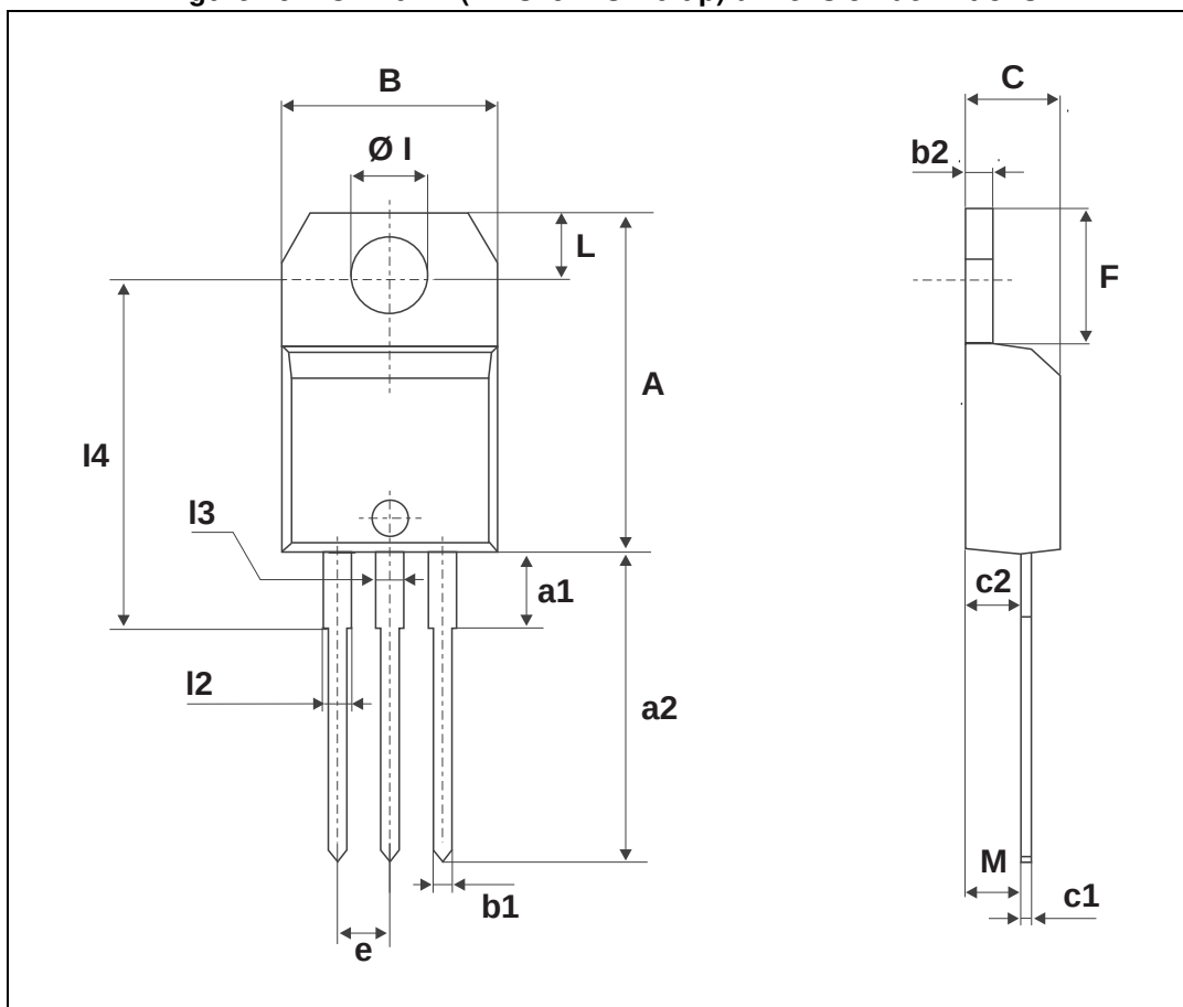
Figure 19. TO-220AB (Nlns. &amp; Ins. 20-up) dimension definitions
