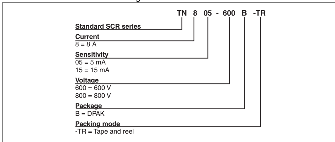
Figure 21. TN8 series
