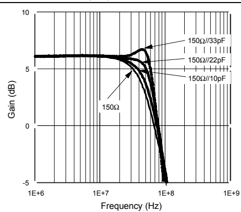
Figure 33. Overshoot function of output capacitance (gain = +2, V_{CC} = \pm 5\text{ V} , T_{amb} = 25\text{ }^\circ\text{C} )
