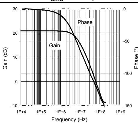
Figure 20. Closed loop gain and phase vs. frequency (gain = +11, V_{CC} = \pm 2.5\text{ V} , R_L = 150\ \Omega , T_{amb} = 25\text{ }^\circ\text{C} )
