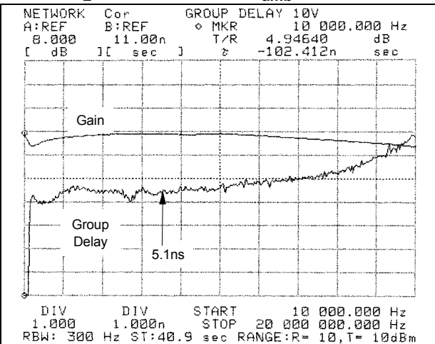
Figure 45. Group delay (gain = 2, V_{CC} = \pm 5 V Z_L = 150 \Omega // 27 pF, T_{amb} = 25^\circ\text{C} )
