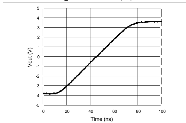
Figure 36. Large signal measurement - positive slew rate (gain = 2, V_{CC} = \pm 5\text{ V} , Z_L = 150\ \Omega \parallel 5.6\text{ pF} )
