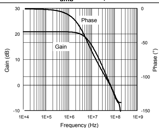
Figure 35. Closed loop gain and phase vs. frequency (gain = +11, V_{CC} = \pm 5\text{ V} , R_L = 150\ \Omega , T_{amb} = 25\text{ }^\circ\text{C} )
