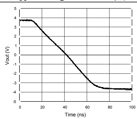
Figure 37. Large signal measurement - negative slew rate (gain = 2, V_{CC} = \pm 5\text{ V} , Z_L = 150\ \Omega \parallel 5.6\text{ pF} )
