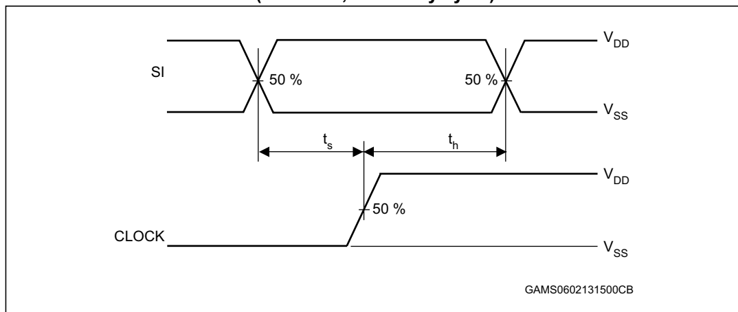
Figure 6. Waveform 2: setup and hold times (SI to CLOCK) ( f = 1\text{ MHz} ; 50 % duty cycle)
