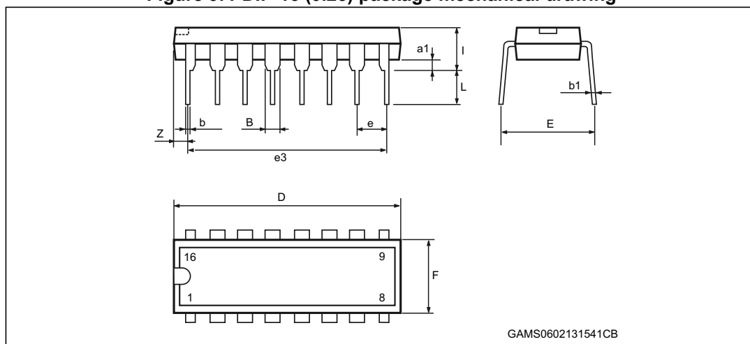
Figure 9. PDIP-16 (0.25) package mechanical drawing
