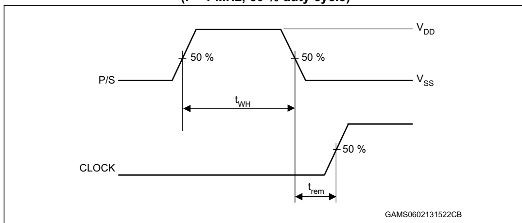
Figure 8. Waveform 4: pulse width and removal time (P/S to clock) ( f = 1\text{ MHz} ; 50 % duty cycle)
