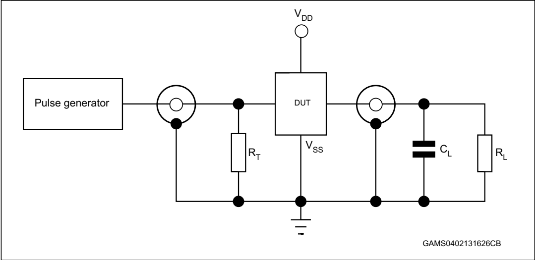
Figure 4. Test circuit
