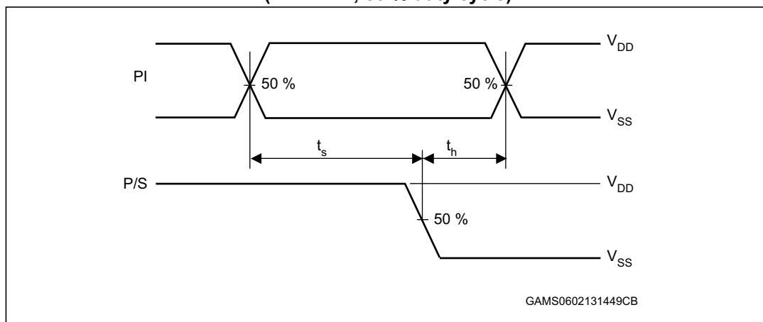
Figure 7. Waveform 3: setup and hold time (PI to P/S) ( f = 1\text{ MHz} ; 50 % duty cycle)
