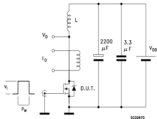
Figure 17. Unclamped Inductive load test circuit
