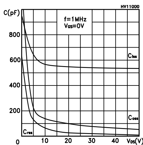
Figure 9. Capacitance variations
