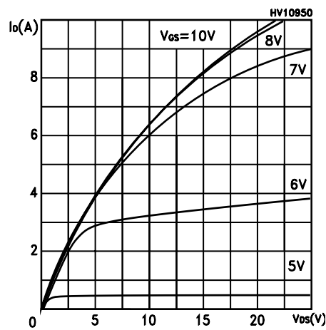
Figure 5. Output characteristics
