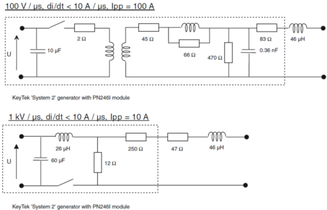
Figure 11. Test circuit 2 for I_{BO} and V_{BO} parameters
