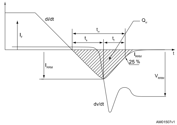
Figure 20. Switching waveform
