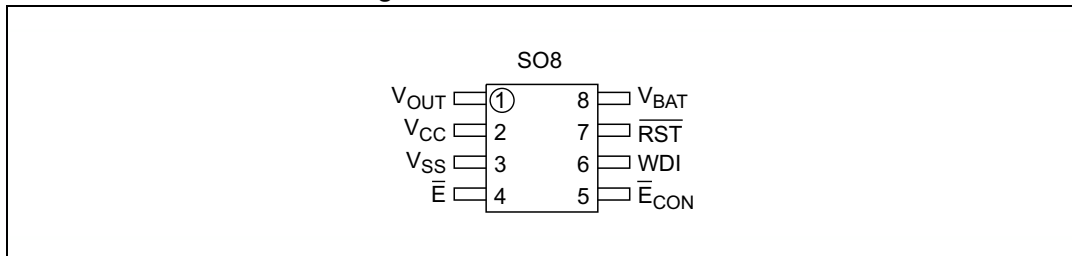
Figure 6. STM818 connections
