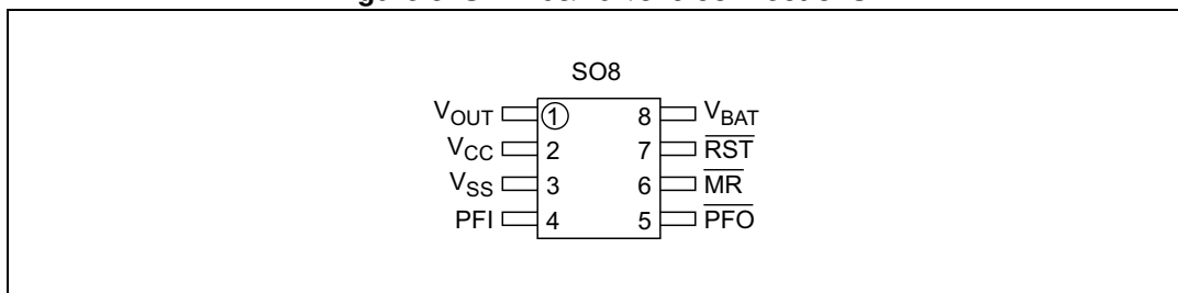
Figure 5. STM703/704/819 connections
