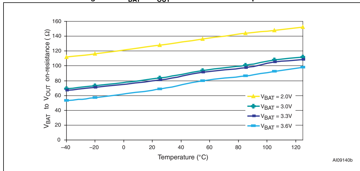
Figure 18. V_{BAT} to V_{OUT} on-resistance vs. temperature
