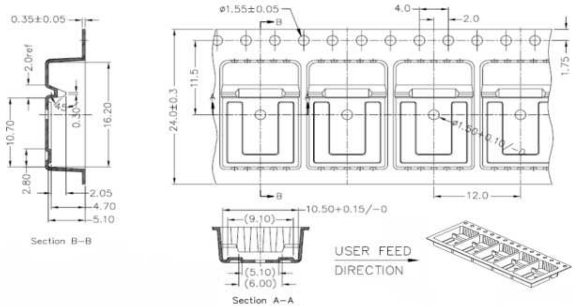
Figure 29. H 2 PAK-2 tape drawing (dimensions are in mm)
