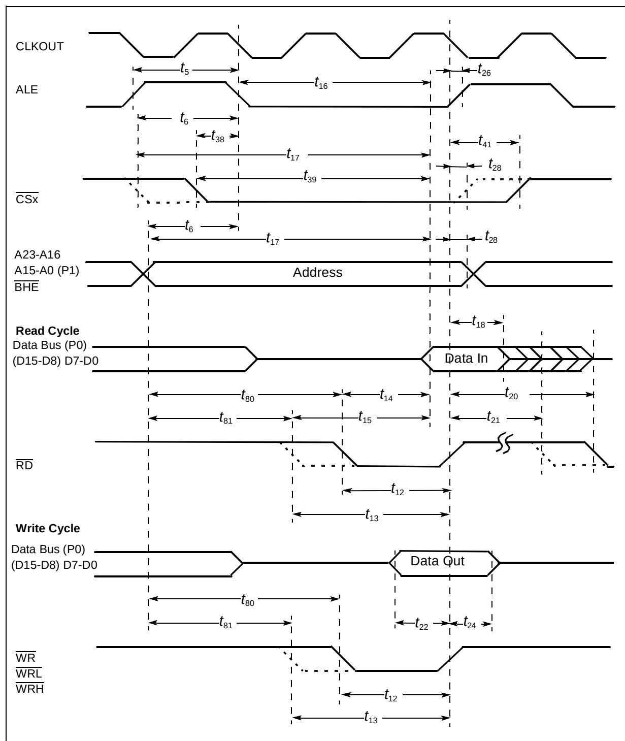
Figure 76 : External Memory Cycle: Demultiplexed Bus, With / Without Read / Write Delay, Extended
