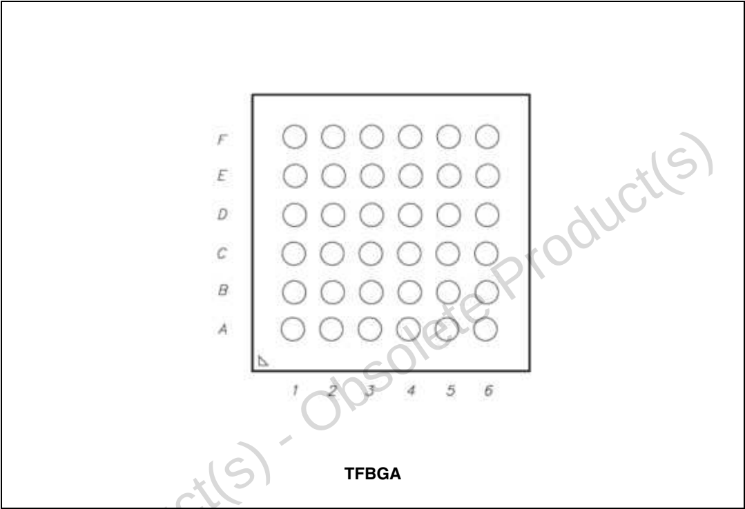
Figure 2. Pin connection
