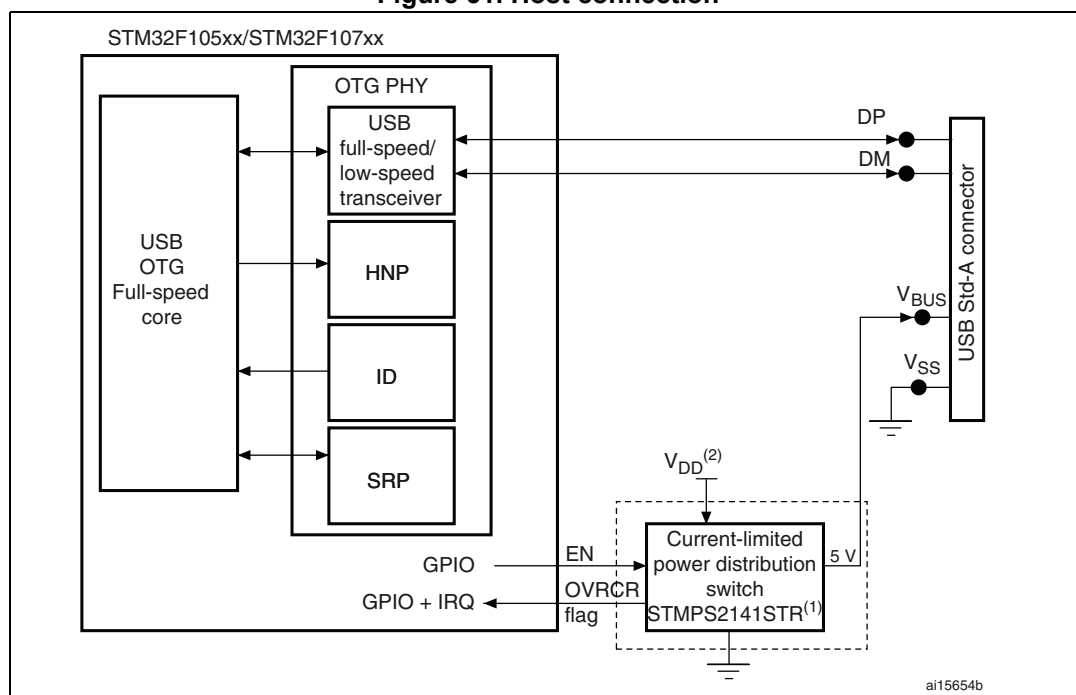
Figure 51. Host connection
