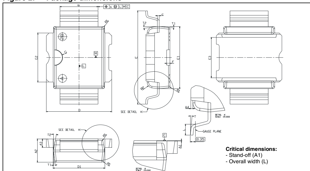
Figure 2. Package dimensions
