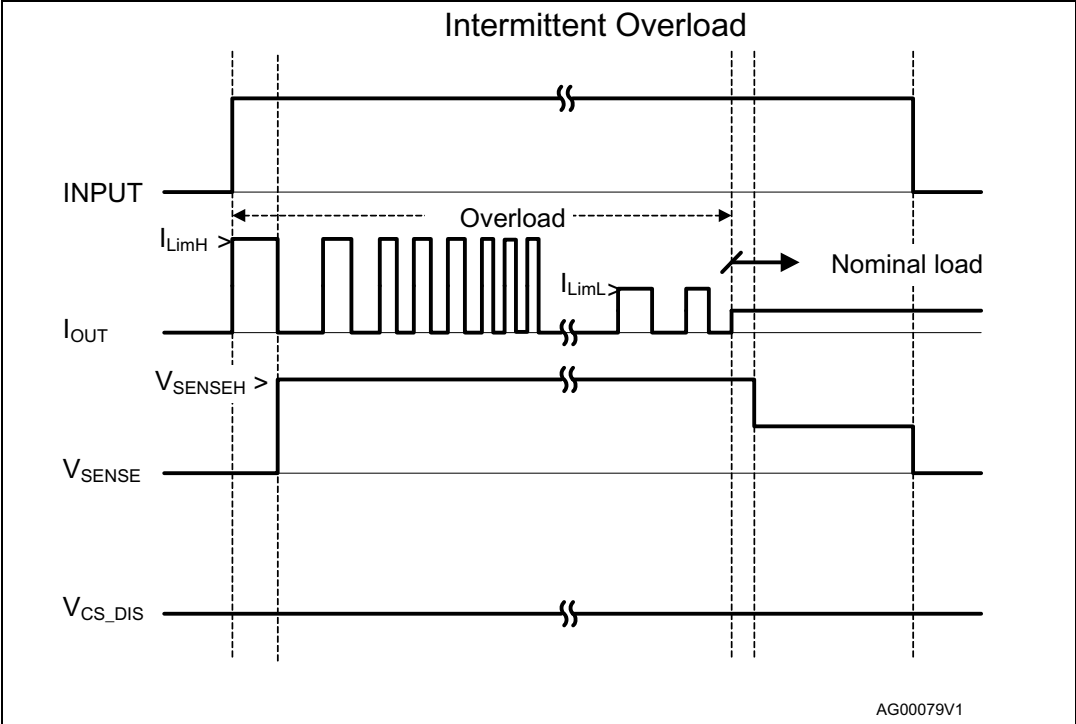
Figure 12. Intermittent overload
