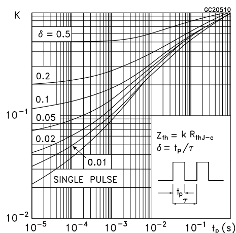
Figure 4. Normalized transient thermal impedance for TO-220
