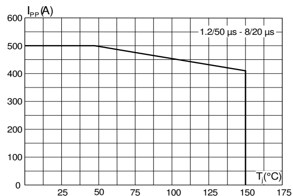
Figure 3: Peak pulse current versus initial junction temperature
