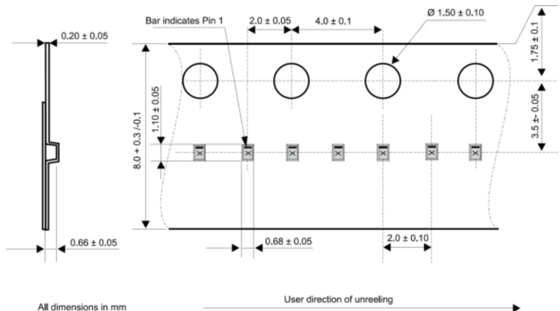
Figure 17. Tape outline
