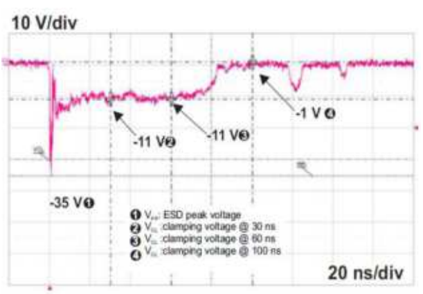
Figure 11. ESD response to IEC 61000-4-2 (-8 kV air discharge)
