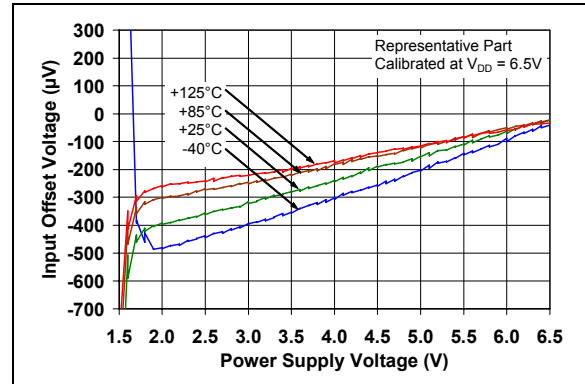
FIGURE 2-4: Input Offset Voltage vs. Power Supply Voltage.
