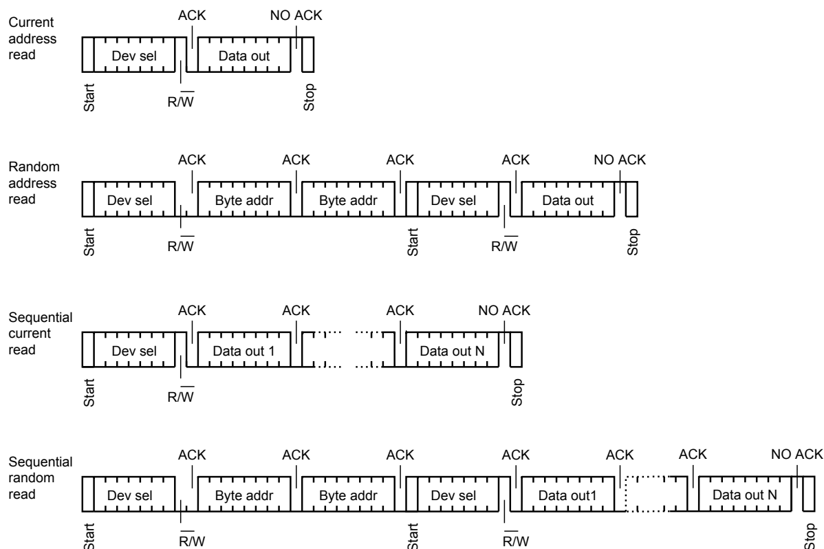
Figure 8. Read mode sequences
