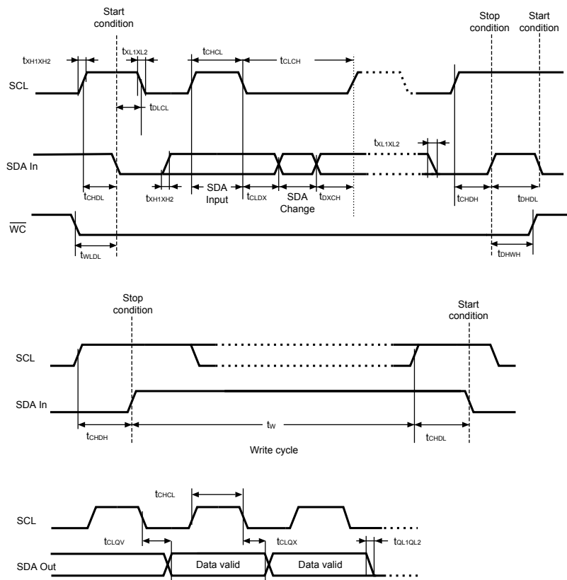
Figure 12. AC waveforms
