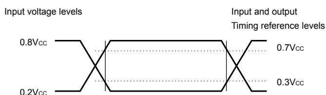
Figure 9. AC measurement I/O waveform
