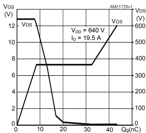
Figure 11. Typical gate charge characteristics
