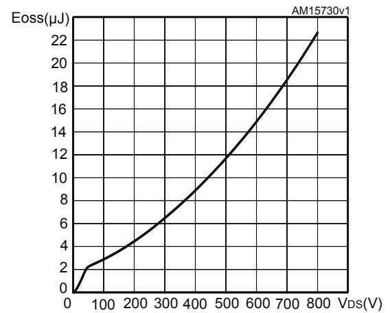
Figure 14. Typical output capacitance stored energy
