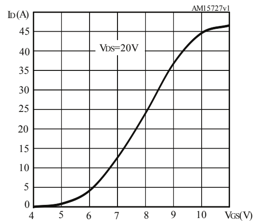
Figure 10. Typical transfer characteristics
