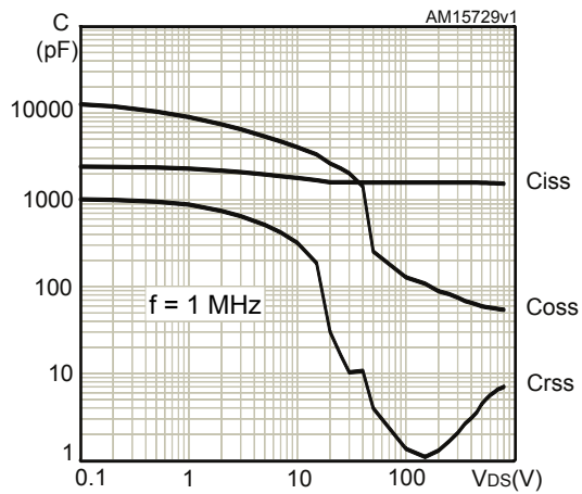
Figure 13. Typical capacitance characteristics
