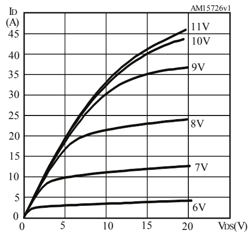
Figure 9. Typical output characteristics
