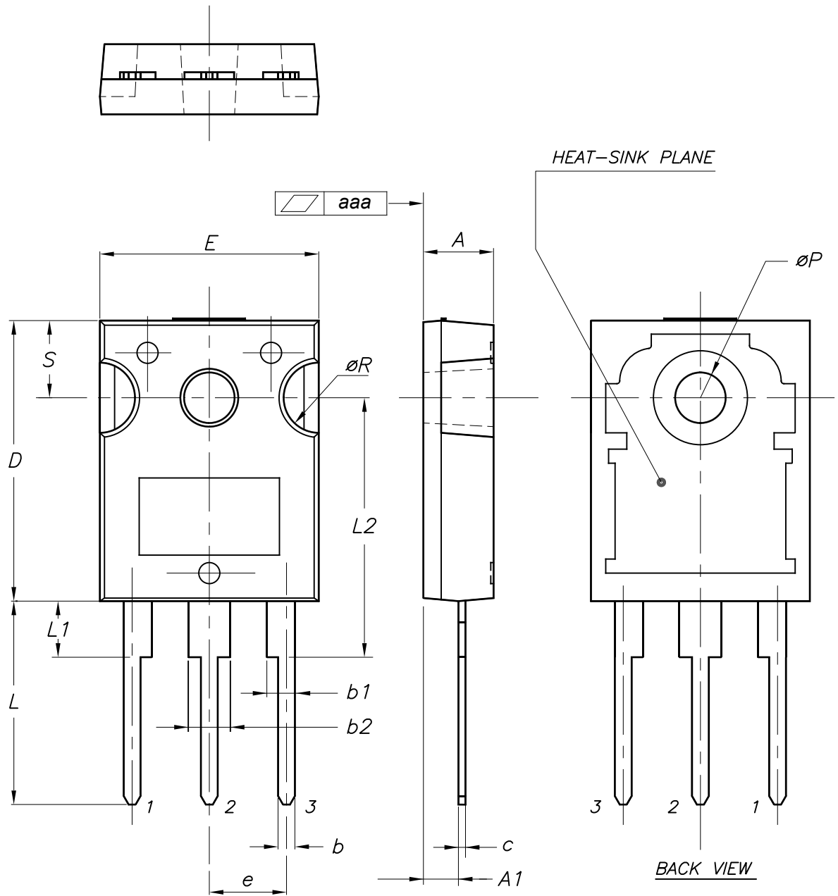
Figure 26. TO-247 package outline
