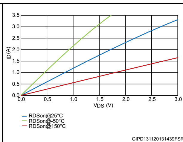
Figure 9. Simulated curves at V_{GS} = 10 V
