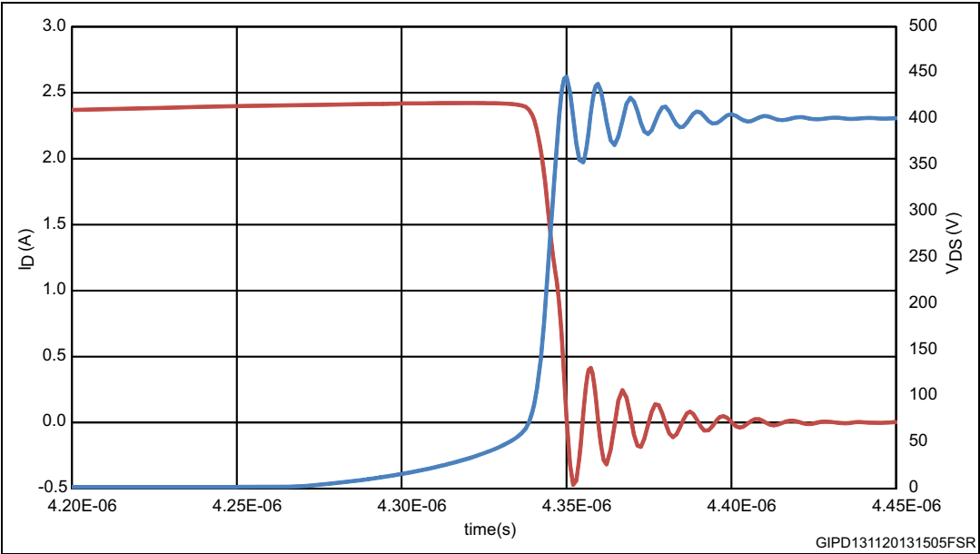
Figure 17. Switching on inductive load - simulated waveforms
