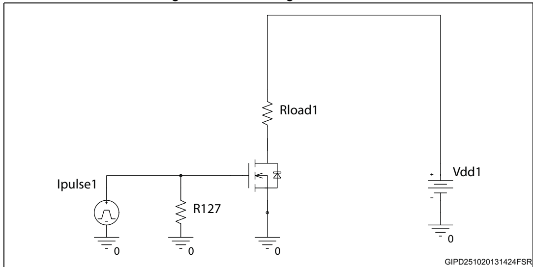
Figure 13. Gate charge - schematic
