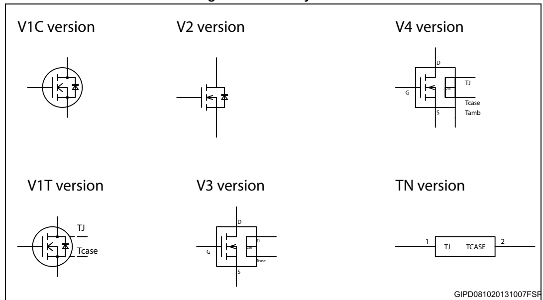
Figure 2. Model symbols
