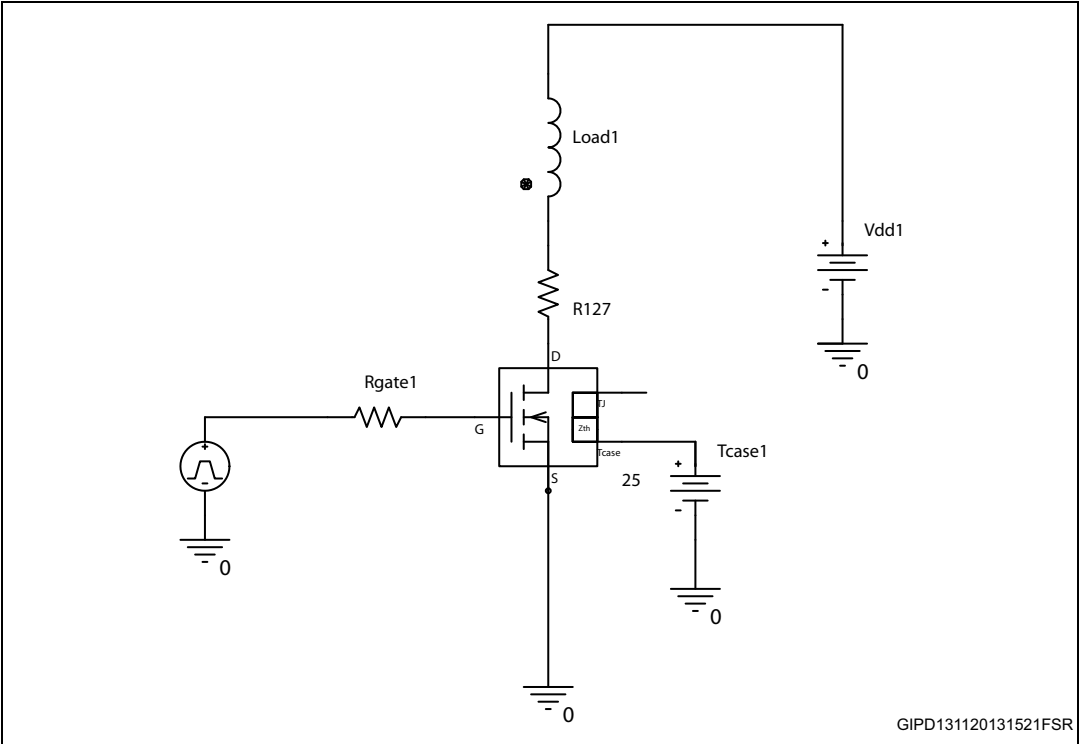
Figure 23. Unclamped inductive switching - schematic
