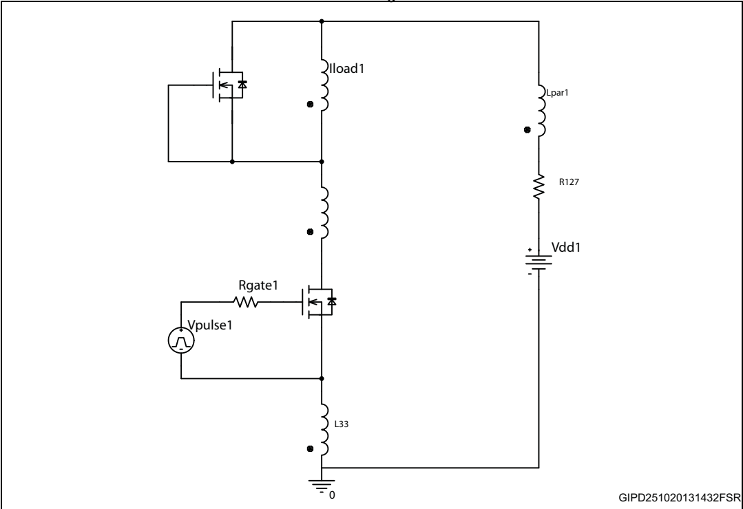
Figure 19. E_{off} vs R_{gate} - schematic
