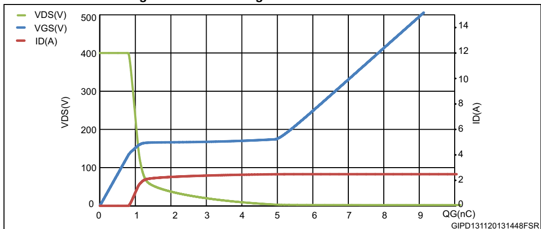
Figure 14. Gate charge - simulated waveforms
