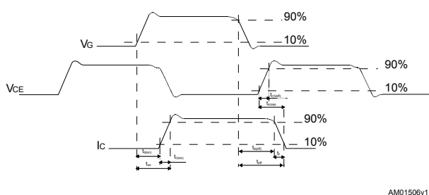
Figure 30. Switching waveform
