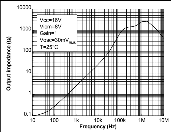
Figure 26. Output impedance vs. frequency in closed loop configuration
