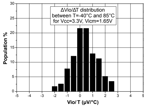
Figure 8. Input offset voltage temperature coefficient distribution
