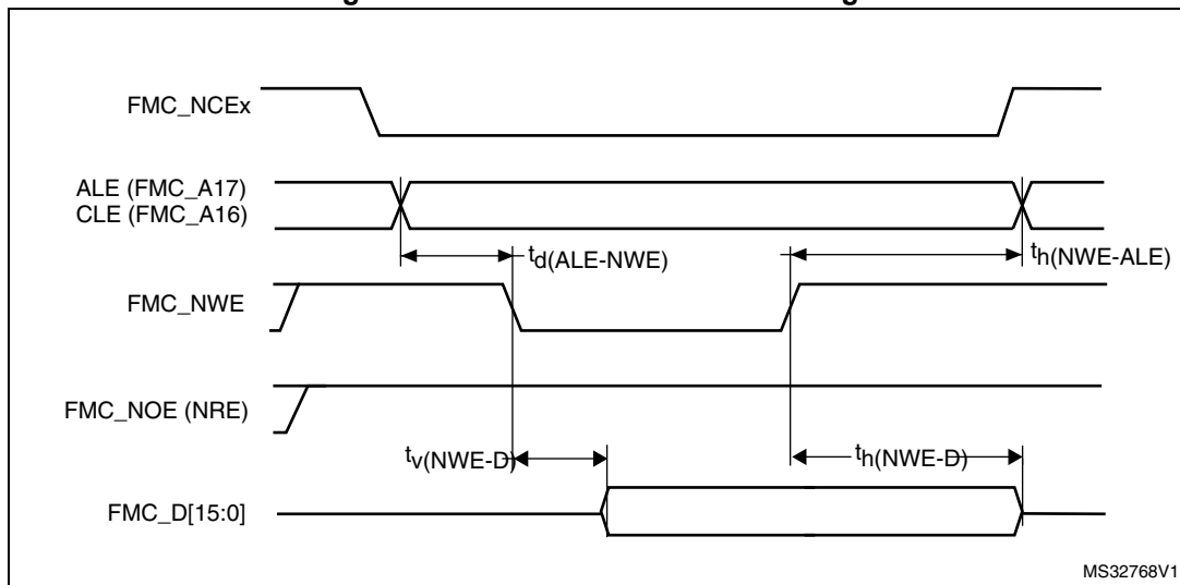
Figure 35. NAND controller write timings
