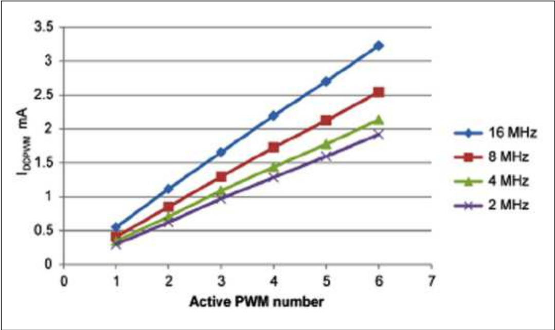
Figure 15. PWM current consumption with f_{SMED} = HSI f_{PWM} = 0.5 MHz at V_{DD}/V_{DDA} = 3.3 V
