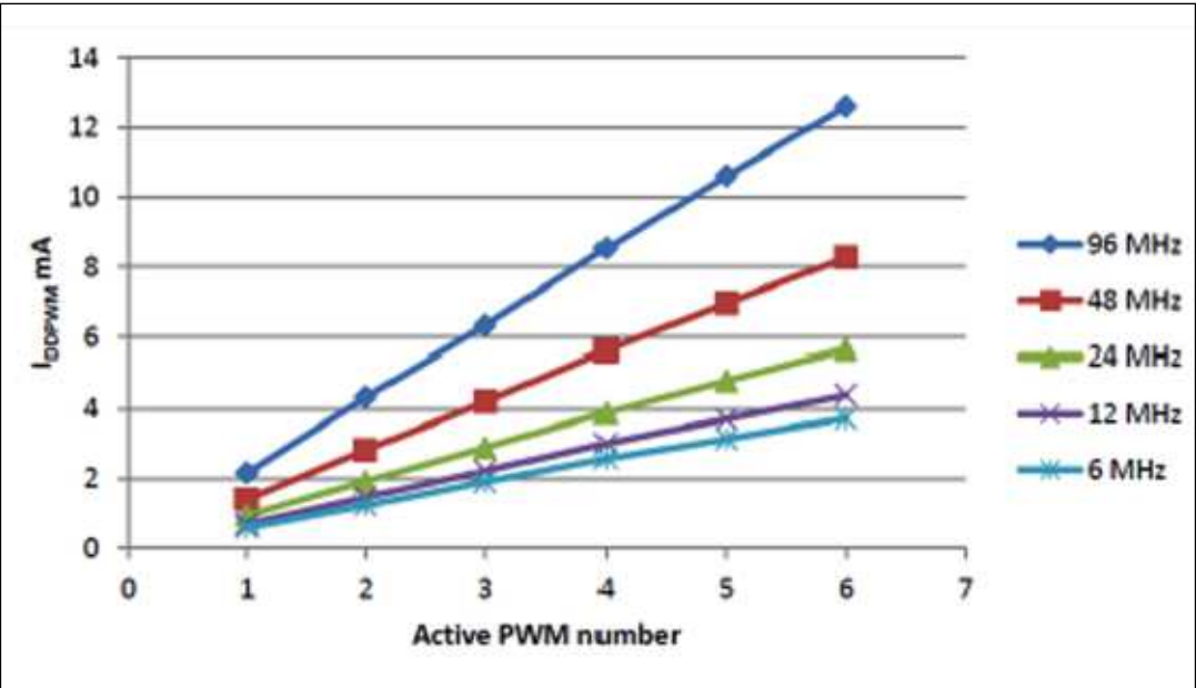
Figure 14. PWM current consumption with f_{\text{SMED}} = \text{PLL } f_{\text{PWM}} = 0.5\text{ MHz} at V_{\text{DD}}/V_{\text{DDA}} = 5\text{ V}
