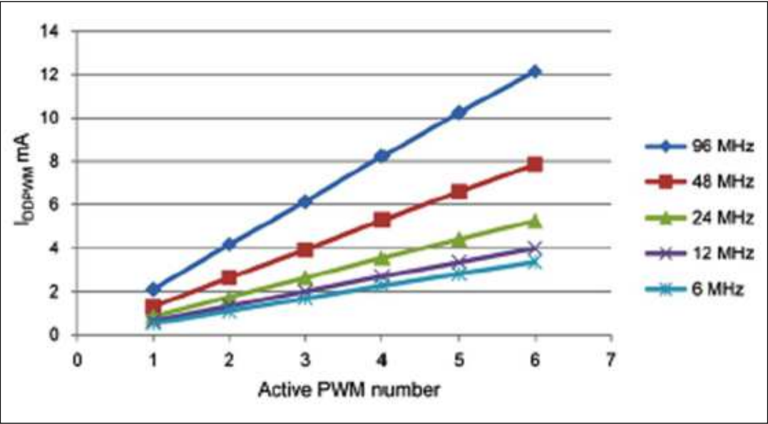
Figure 13. PWM current consumption with f_{\text{SMED}} = \text{PLL } f_{\text{PWM}} = 0.5\text{ MHz} at V_{\text{DD}}/V_{\text{DDA}} = 3.3\text{ V}
