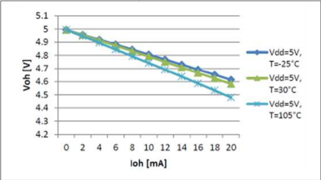
Figure 29. V_{OH} high speed pad at 5 V
