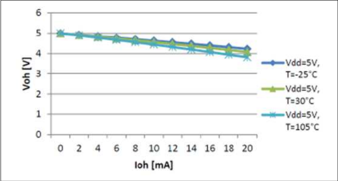
Figure 25. V_{OH} fast pad at 5 V
