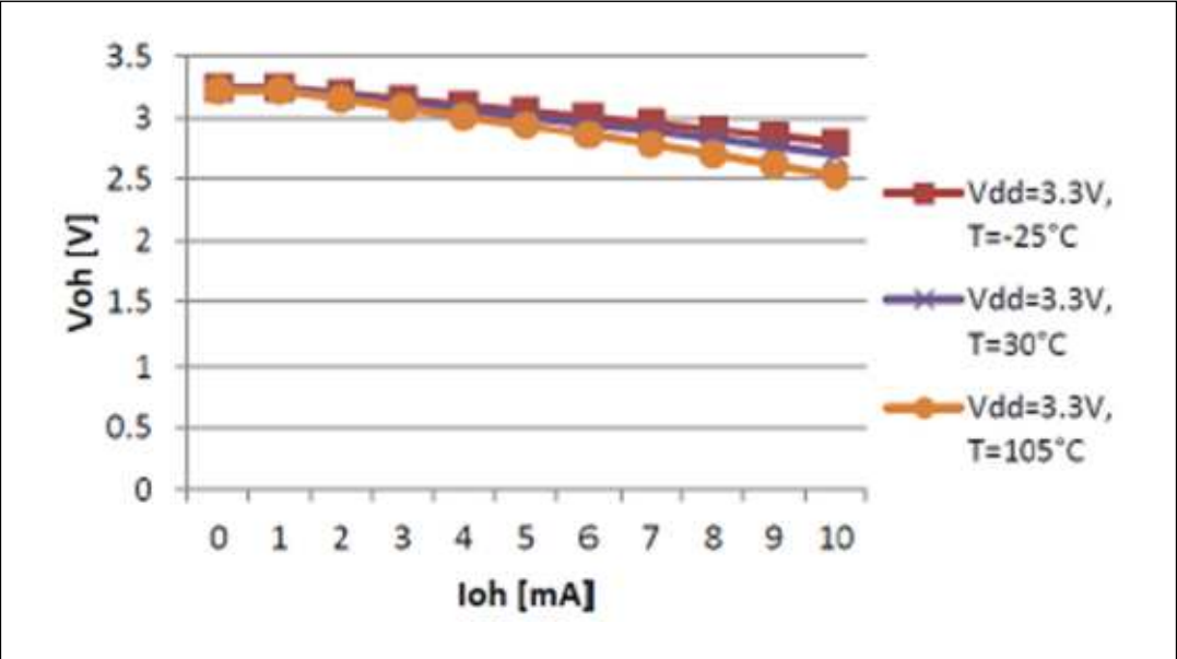
Figure 23. V_{OH} fast pad at 3.3 V
