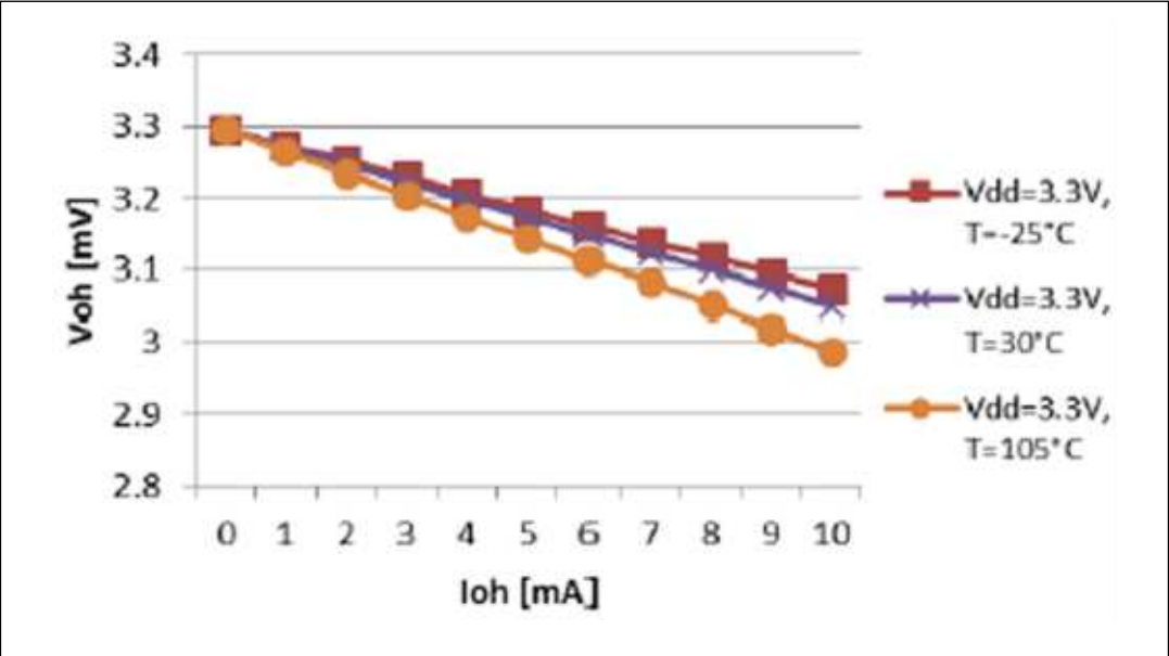
Figure 27. V_{OH} high speed pad at 3.3 V
