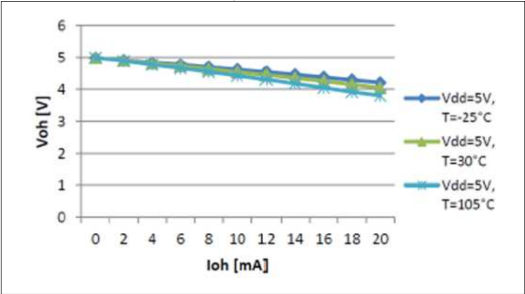
Figure 21. V_{OH} standard pad at 5 V
