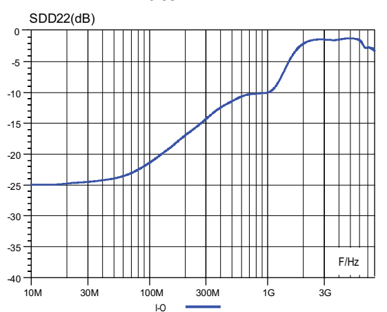
Figure 7. Return loss versus frequency ( Z_{0\text{ com}} = 50\ \Omega )
