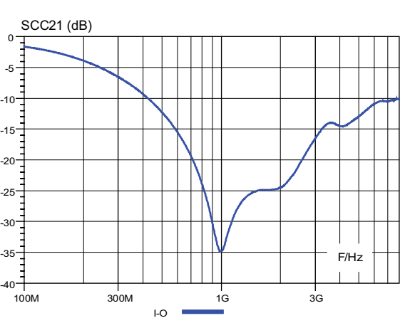
Figure 5. Common mode attenuation versus frequency ( Z_{0\text{ com}} = 50\ \Omega )
