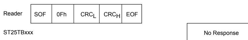
Figure 32. Completion frame exchange between reader and ST25TB04K
