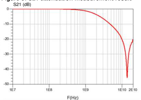
Figure 8: S21 attenuation measurement result
