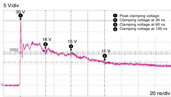
Figure 5: ESD response to IEC 61000-4-2 (+8 kV contact discharge)
