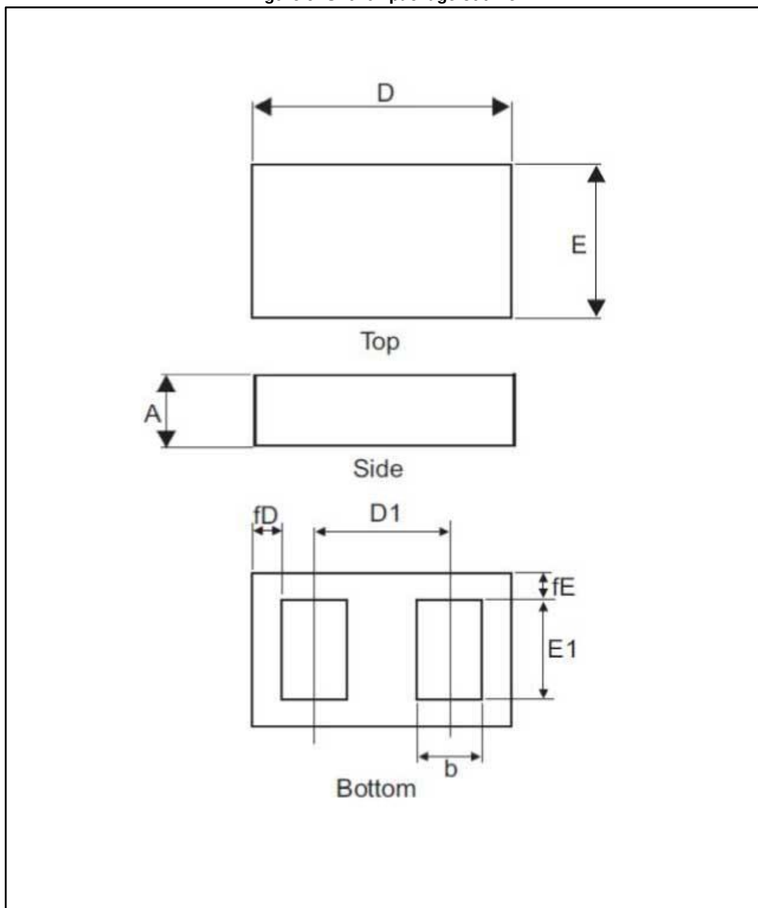
Figure 9: ST0201 package outline
