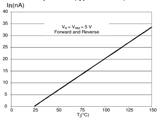
Figure 3: Leakage current versus junction temperature (typical values)
