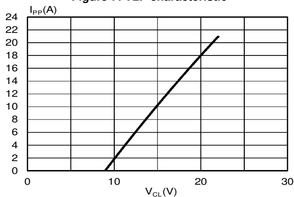
Figure 7: TLP characteristic
