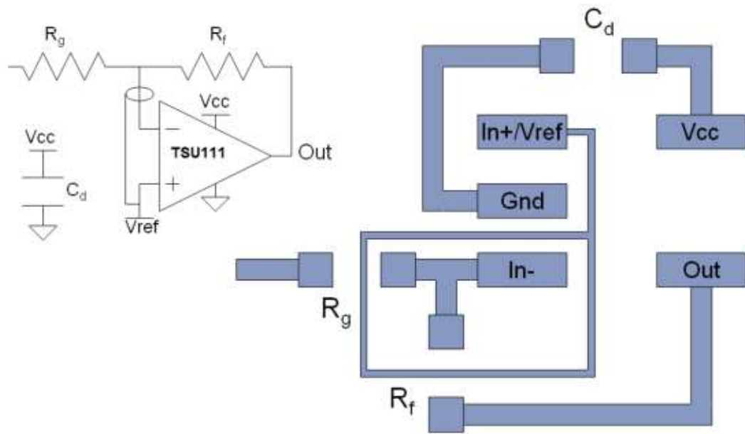
Figure 35. Guarding on the PCB
