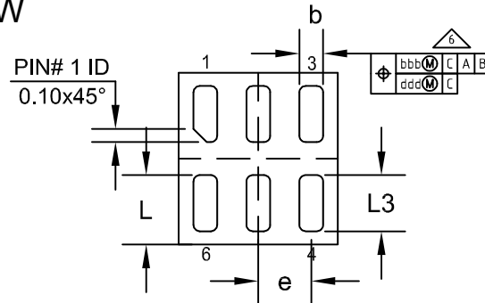
Figure 65. DFN6 1.2 x 1.3 package outline
