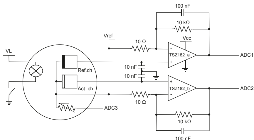
Figure 62. Principle schematic
