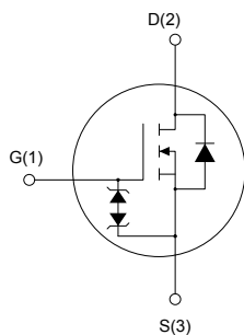
TO-220FP
