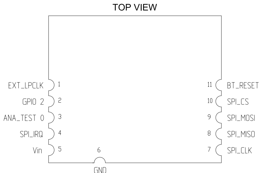
Figure 12. Pin assignment
