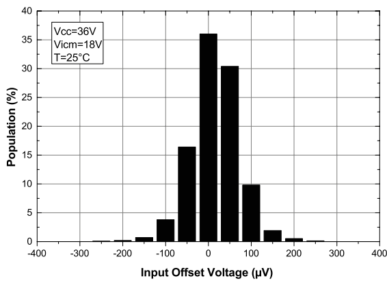
Figure 5. Input offset voltage distribution at V_{CC} = 36\text{ V} TSB711A, TSB712A
