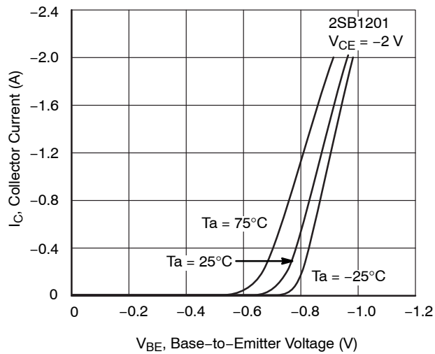
Figure 6. I_C - V_{BE}
