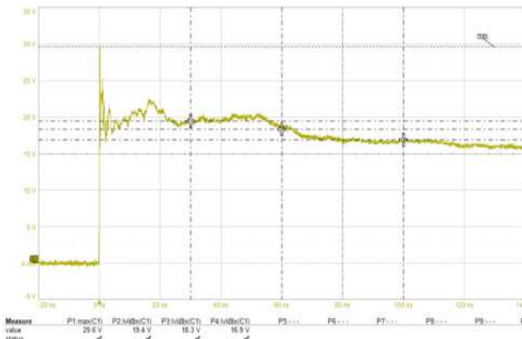
Figure 4. ESD response to IEC 61000-4-2 (+8 kV contact discharge)
