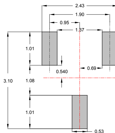
Figure 14. SOT23-3L footprint in mm
