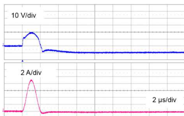
Figure 11. Slow transient pulse 2a ( U_s = +85\text{ V} )
