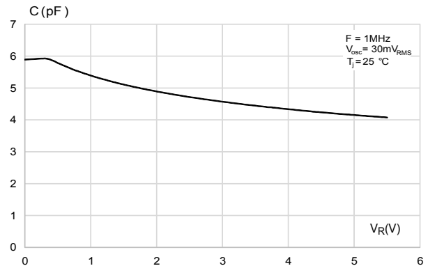
Figure 3. Junction capacitance versus applied voltage (typical values)
