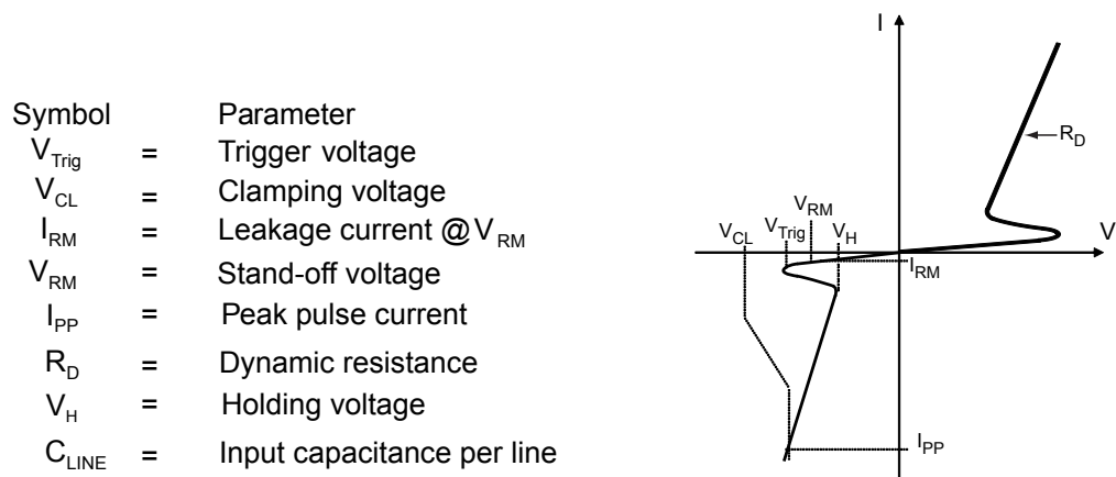
Figure 1. Electrical characteristics (definitions)
