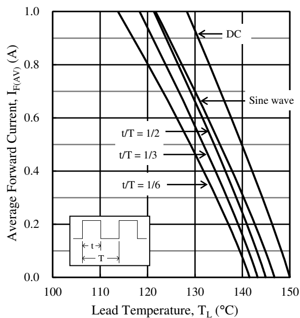
Figure 3. I_{F(AV)} vs. T_L^{(2)} ( T_J = 150 °C, V_R = 200 V)
