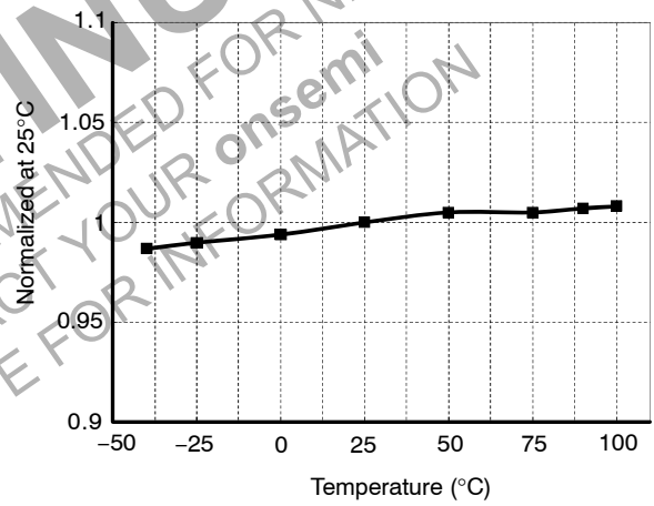
Figure 13. V_{\text{CSsH}} vs. Temperature
