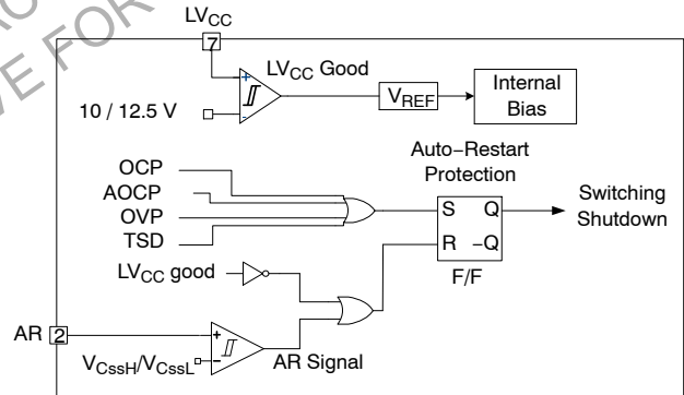
Figure 22. Protection Blocks
