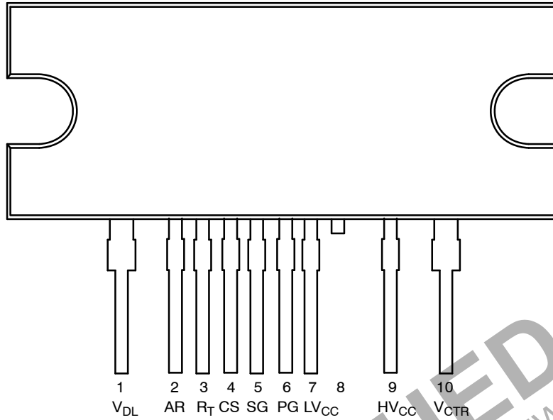
Figure 3. Pin Configuration
