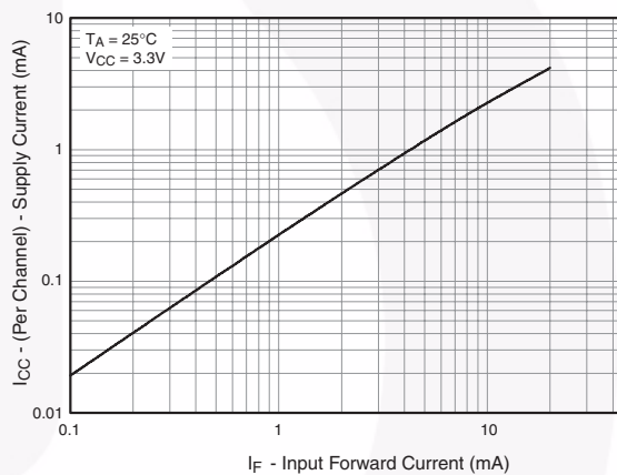
Fig. 4 Supply Current vs Input Forward Current
