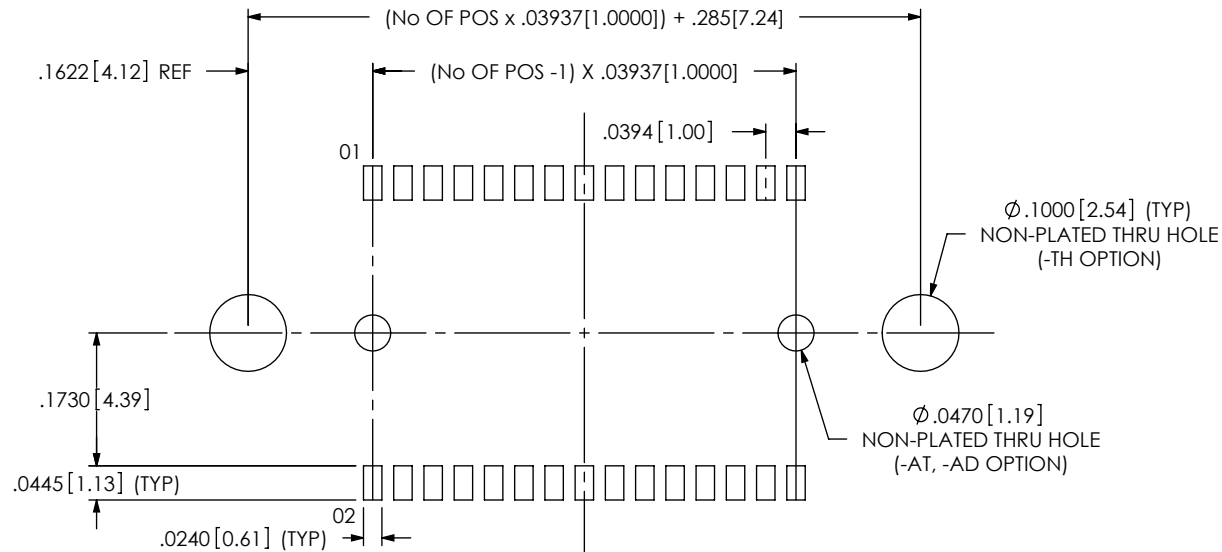
FIG 1 FOR -10, -20, -30 POS (THREADED) OR -05 THRU -50 POS (NON-THREADED)
