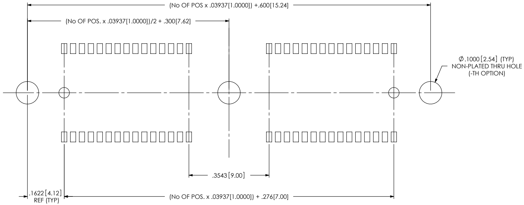
FIG 2 FOR -40 AND -50 POS (THREADED)
