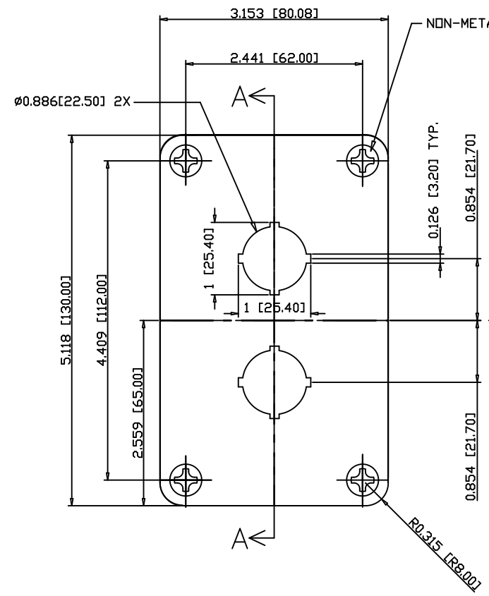
TOP VIEW WITH COVER
