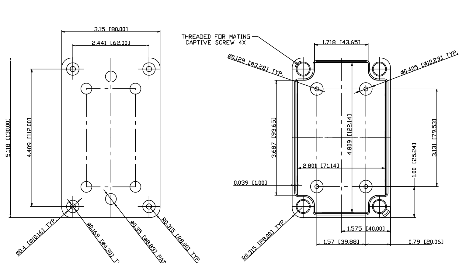
TOP VIEW WITH COVER REMOVED
