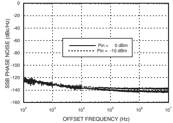
SSB Phase Noise Performance, F_{out} = 15.0 GHz
