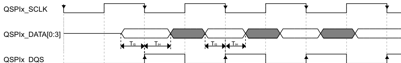
Figure 50. QuadSPI Input/Read Timing (SDR mode with loopback DQS sampling)
