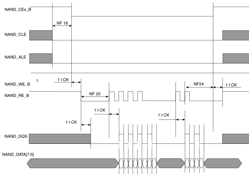
Figure 31. Samsung Toggle Mode Data Read Timing
