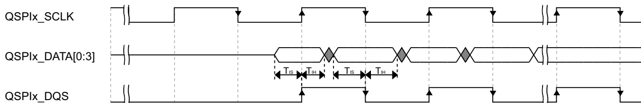
Figure 53. QuadSPI Input/Read Timing (DDR mode with loopback DQS sampling)
