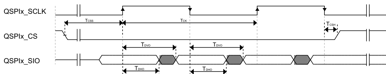
Figure 54. QuadSPI Output/Write Timing (DDR mode)
